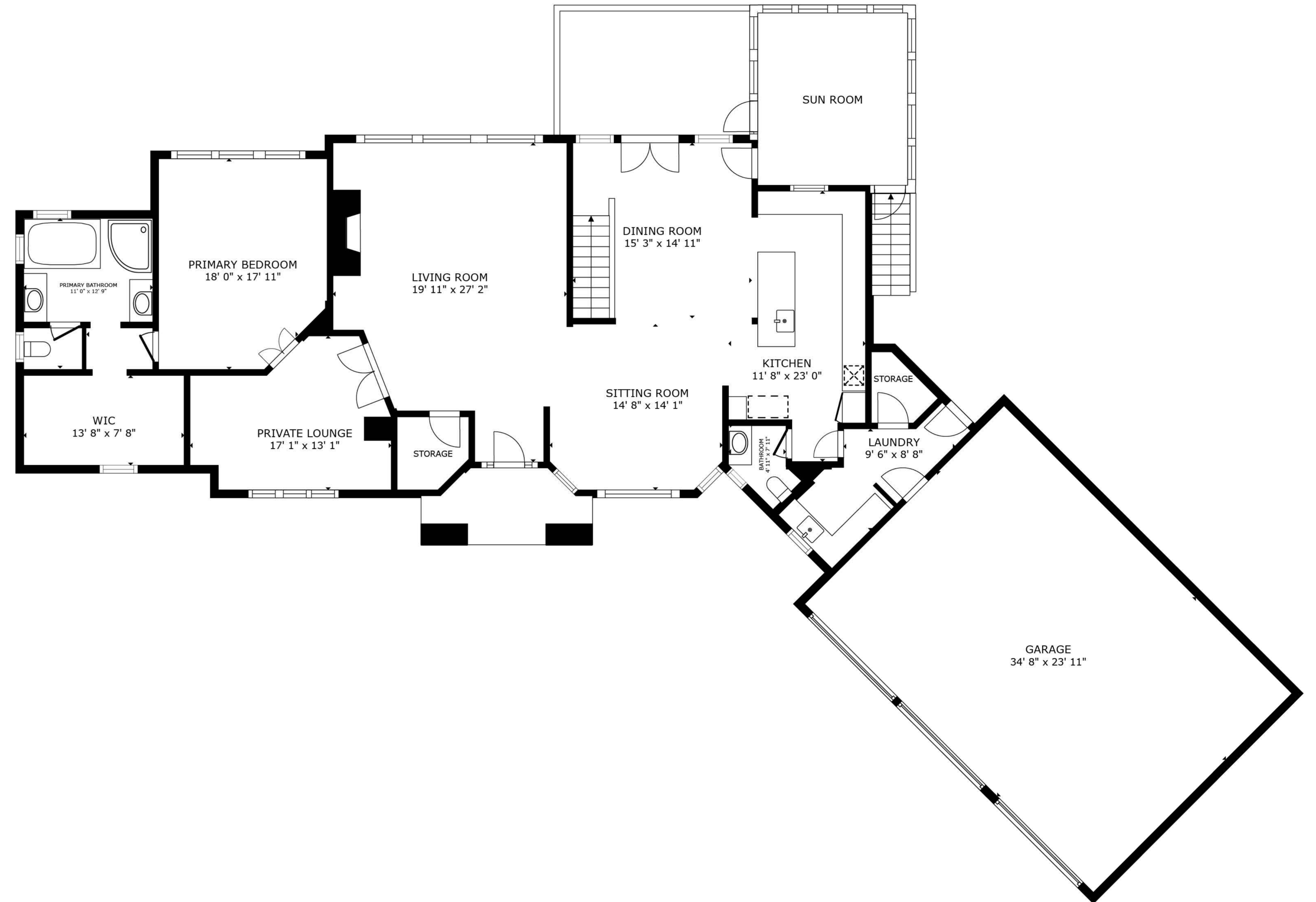
MAIN LEVEL
